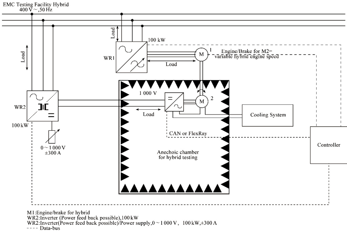
Figure 1 Basic setup of the new absorber chamber
