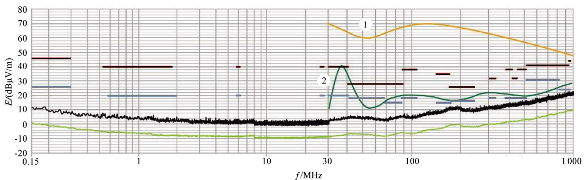
Figure 2 Ambient noises in the chamber with rotating external motor. The chart shows the limit value curves 5 for peak and average assessment as defined in CISPR 25. Curves 1 and 2 during shielding development
