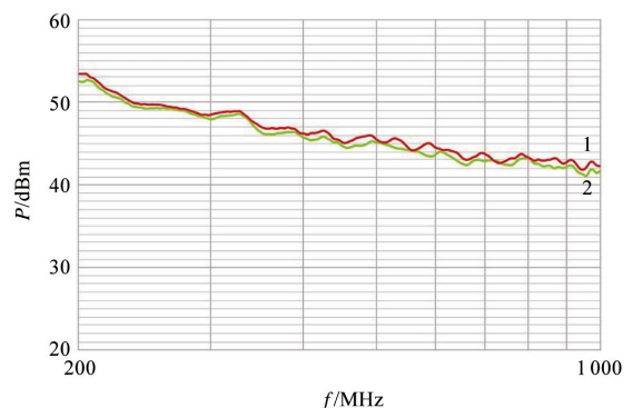
Curve1: reference curve for comparable absorber chamber Curve2: absorber chamber measurement curve for HV components and E drives
